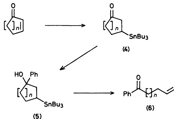
Scheme 2. a; n = 1 b; n = 2 c; n = 3
